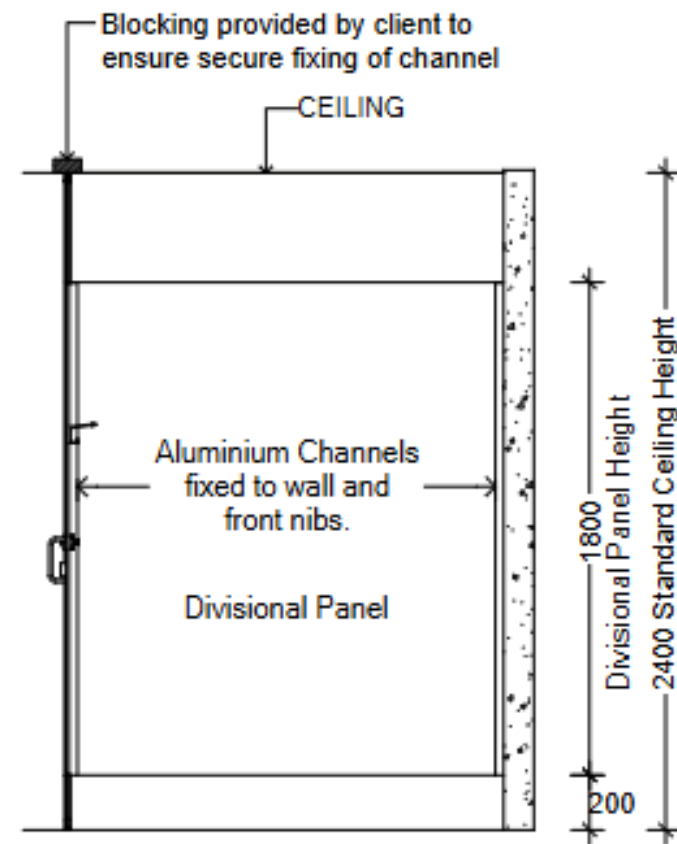
Section
