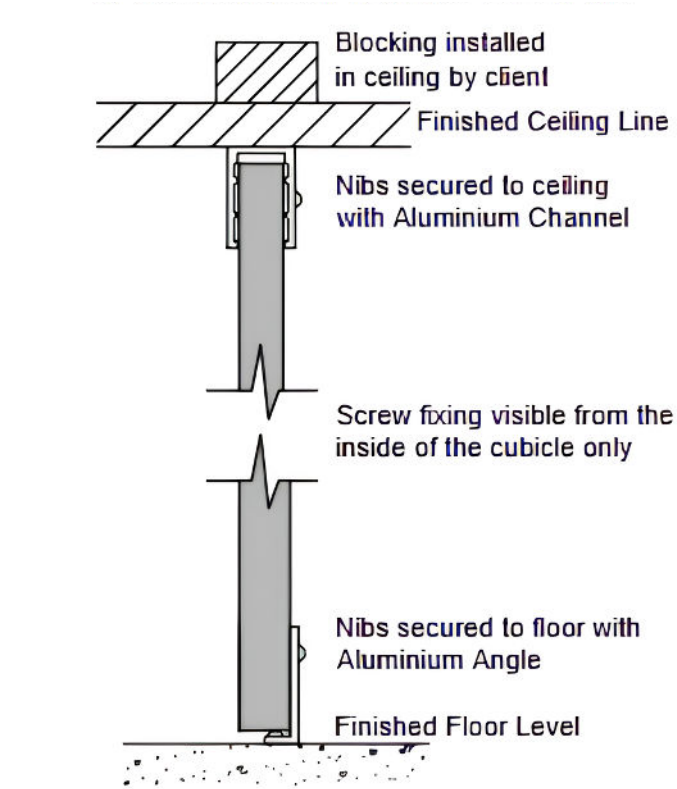
Floor & Ceiling Fixing Detail
