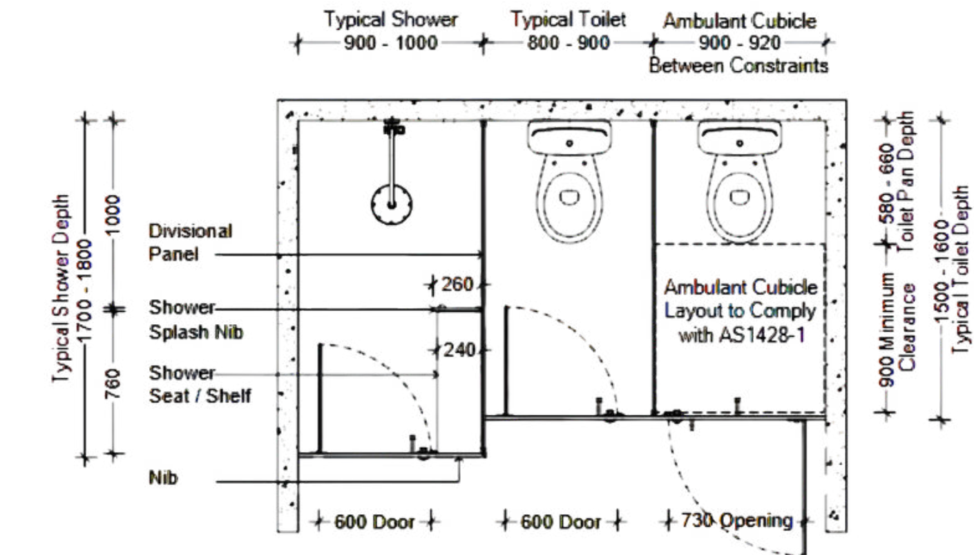
Plan
