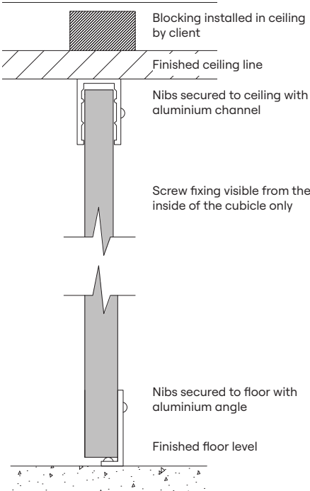
Floor Mounting Detail
