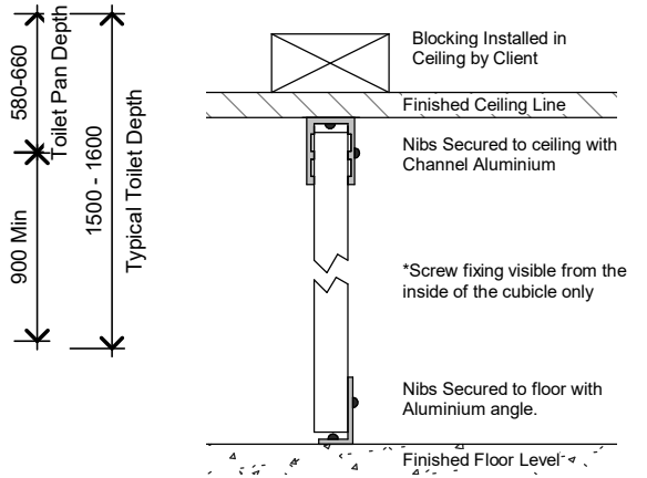
Floor & Ceiling Fixing Detail
