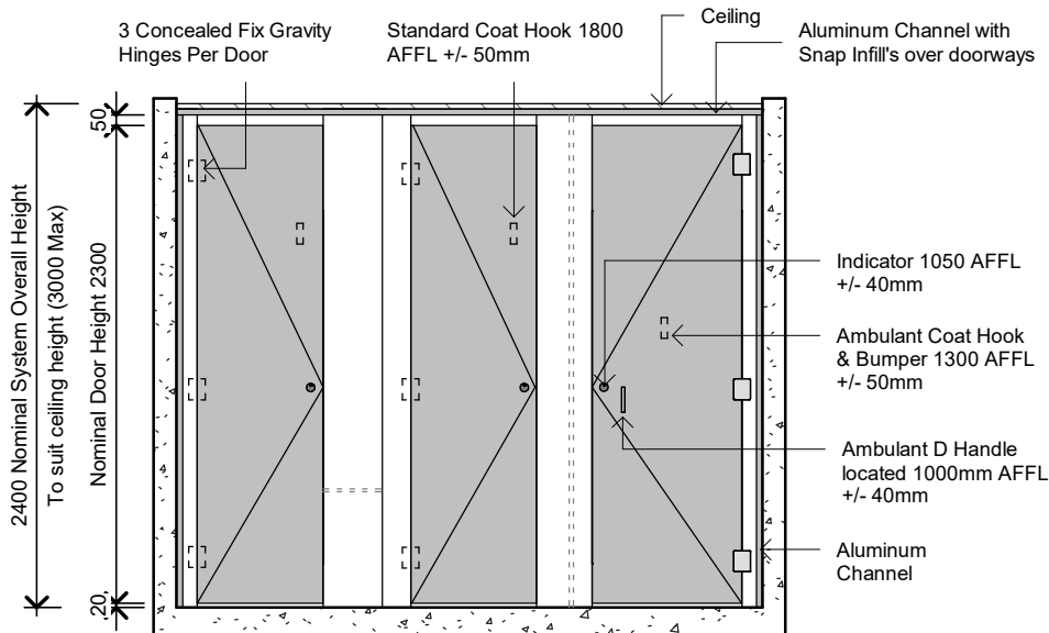
Typical Elevation
