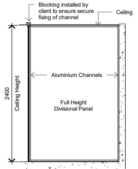
Typical Section
