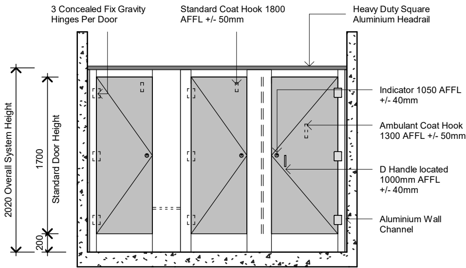
Typical Elevation
