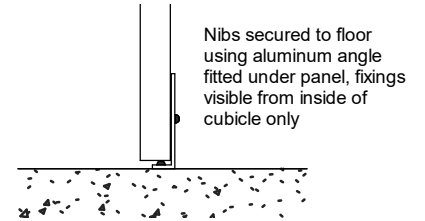
Floor Fixing Detail
