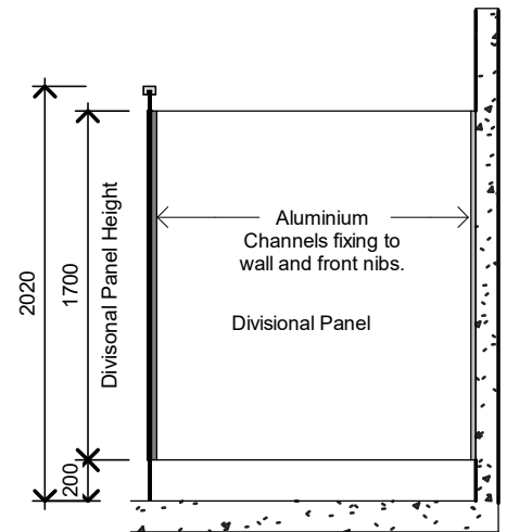
Typical Section
