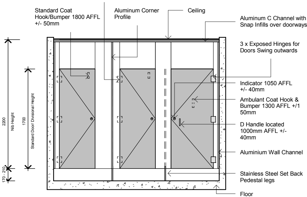
Typical Elevation
