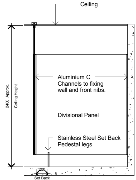
Typical Section
