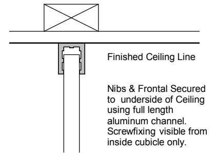
Ceiling Fixing Detail
