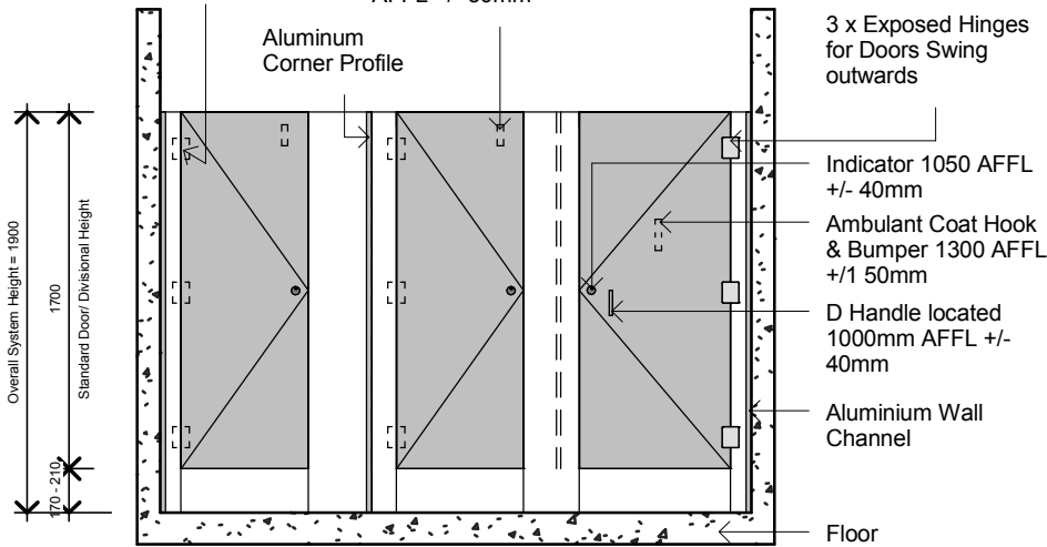
Typical Elevation
