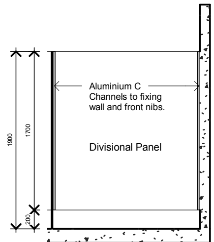
Typical Section
