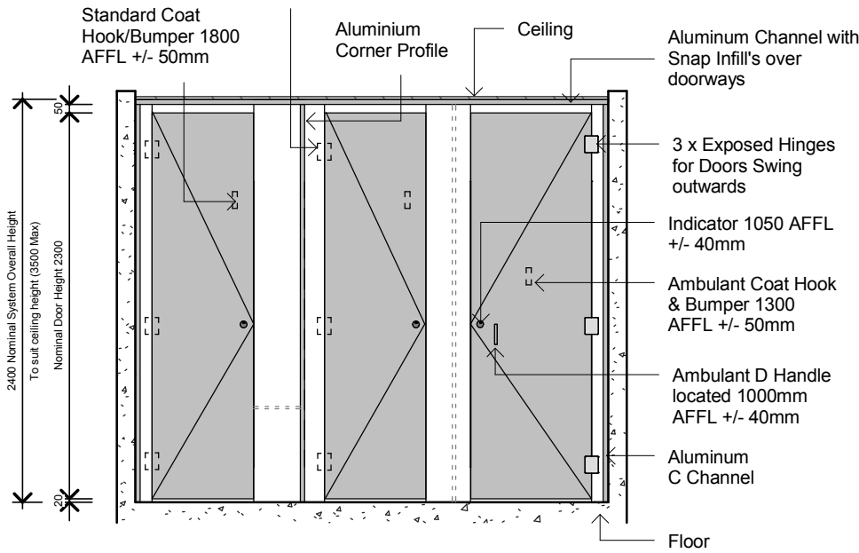
Typical Elevation
