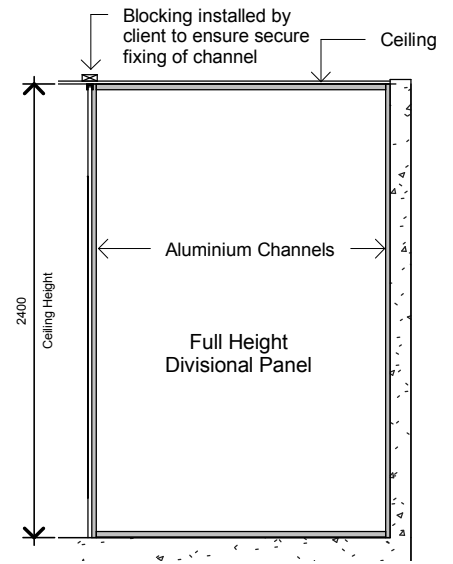
Typical Section
