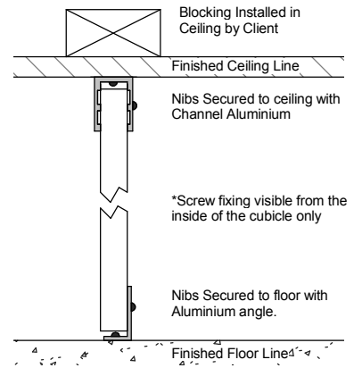
Floor & Ceiling Fixing Detail
