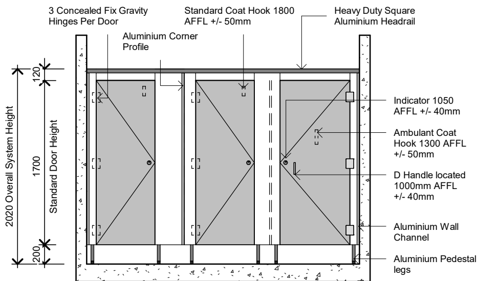
Typical Elevation
