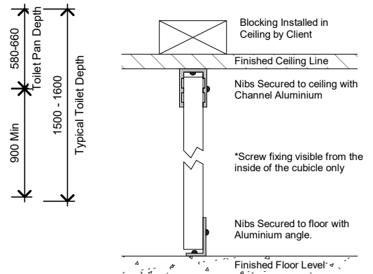
Floor & Ceiling Fixing Detail
