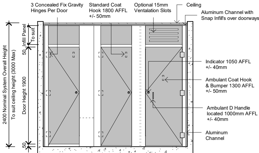
Typical Elevation
