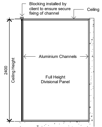
Typical Section
