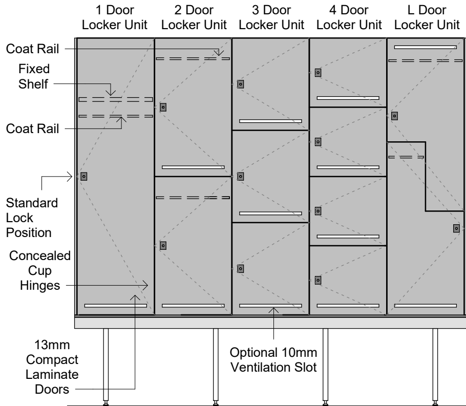
Front Elevation
