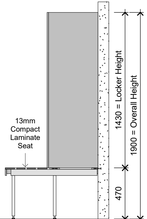
Section
