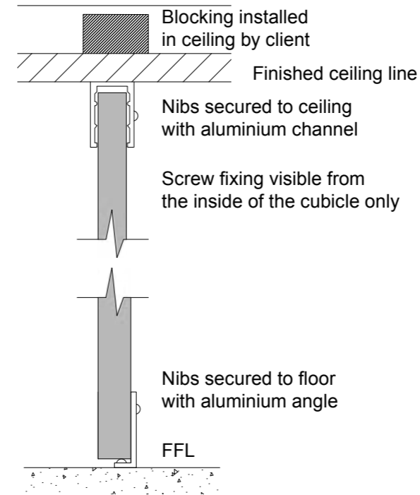
Floor Mounting Detail
