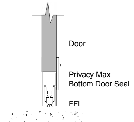
Door Seal Detail
