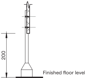
Optional Setback Pedestal Mount Detail
