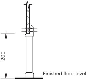
Standard Pedestal Mount Detail
