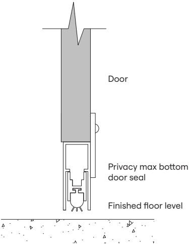
Door Seal Detail
