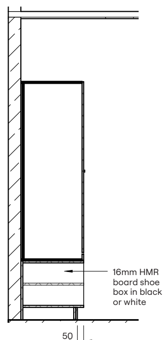
Section
