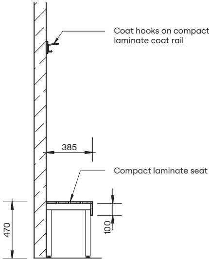
Section
