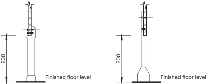
Standard Pedestal Mount Detail
