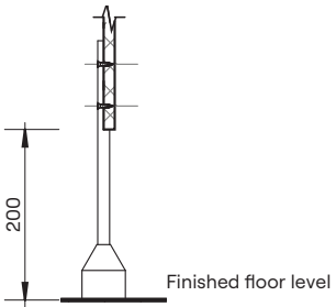
Optional Setback Pedestal Mount Detail
