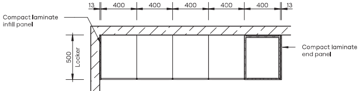
Plan
