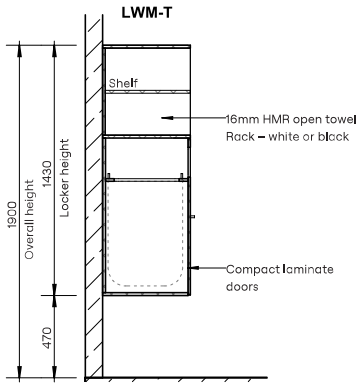
Section
