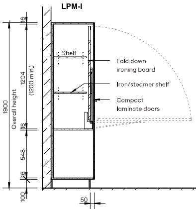
Section
