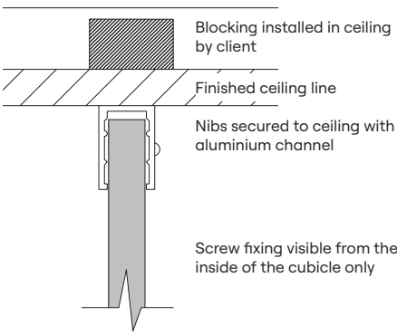
Ceiling Fixing Detail
