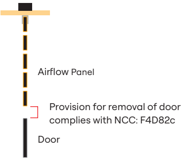
Slotted Panel Detail
