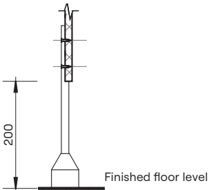
Optional Setback Pedestal Mount Detail
