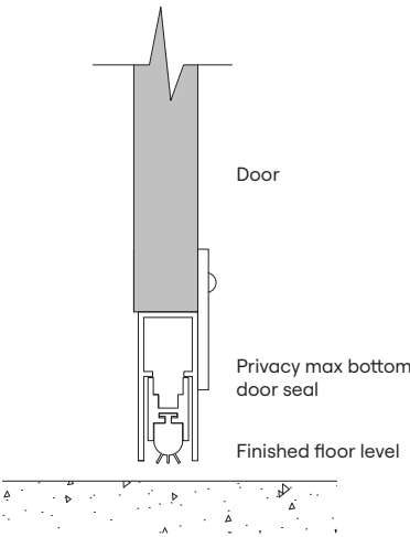
Door Seal Detail
