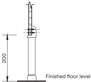
Standard Pedestal Mount Detail
