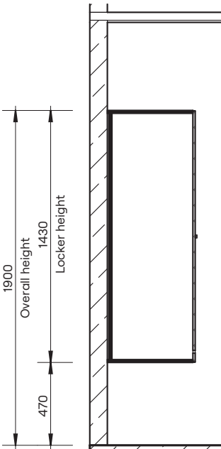
Section
