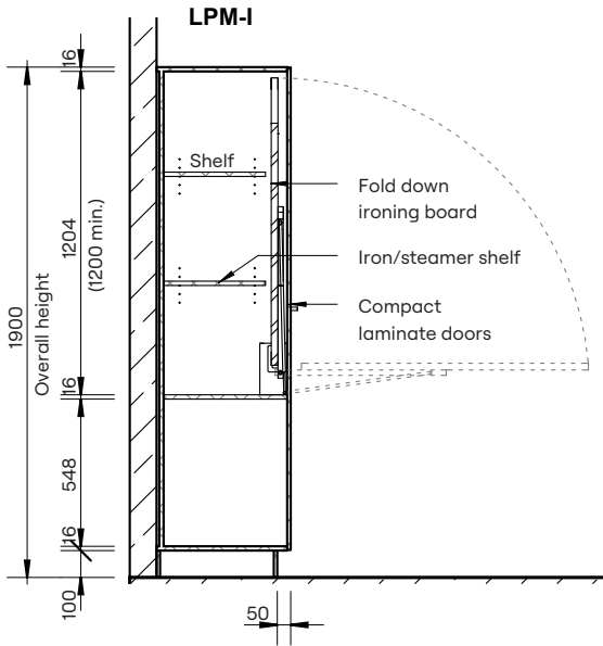
Section
