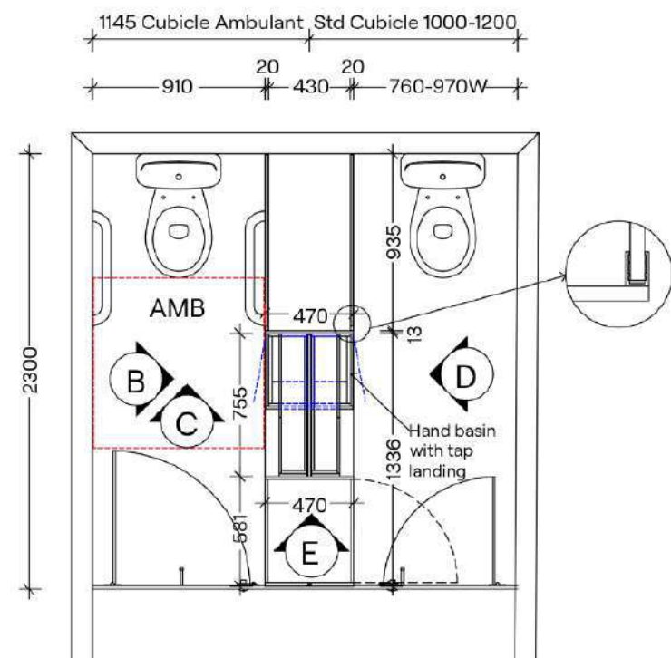
Plan - Optional with Cleaners Cabinet
