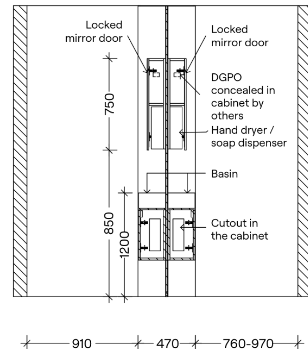
Elevation C
