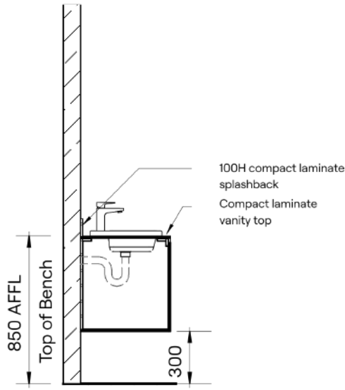
Section
