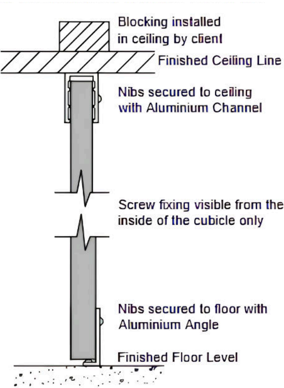
Floor & Ceiling Fixing Detail
