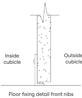
Floor Mounting Detail
