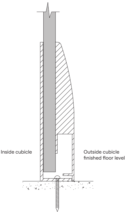
Optional 150mm Skirt Mount Detail
