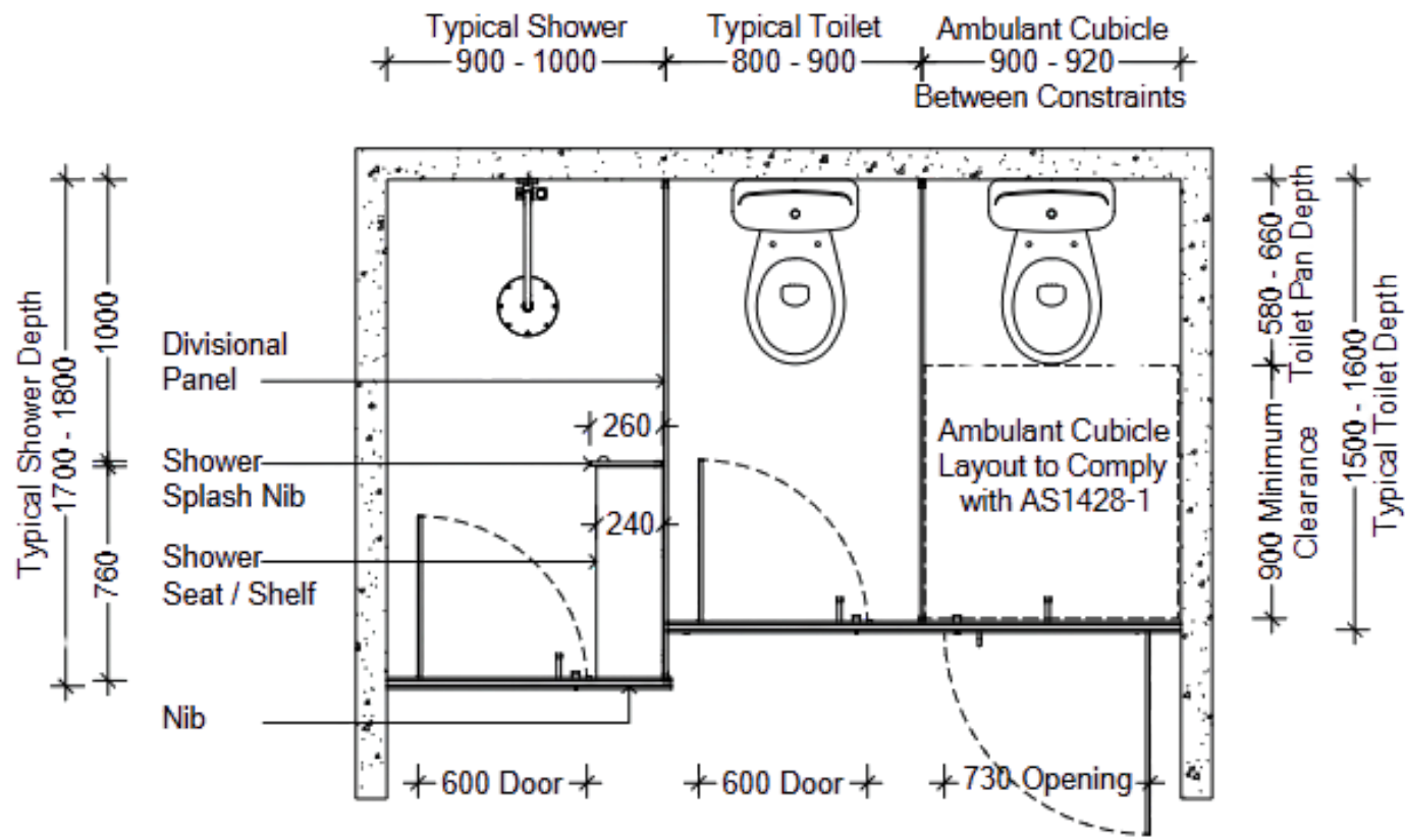
Plan
