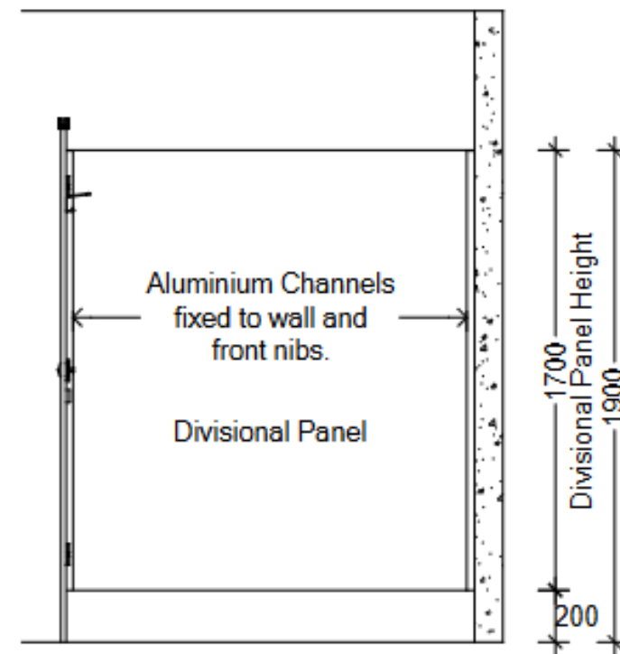
Section
